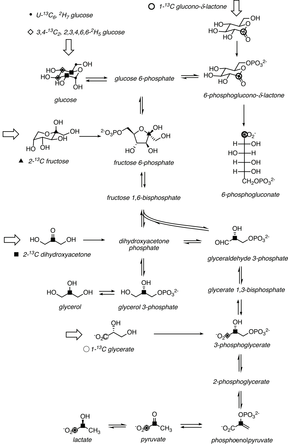
Figure 6.4 HP probes of glucose metabolism
